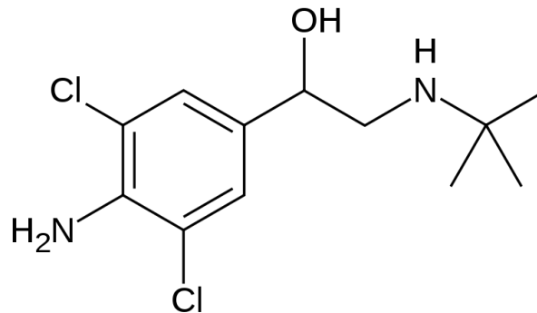
Figure 1. Chemical structure of clenbuterol.
